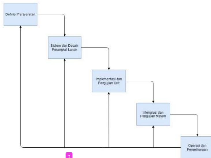
Gambar 1. Model Waterfall
