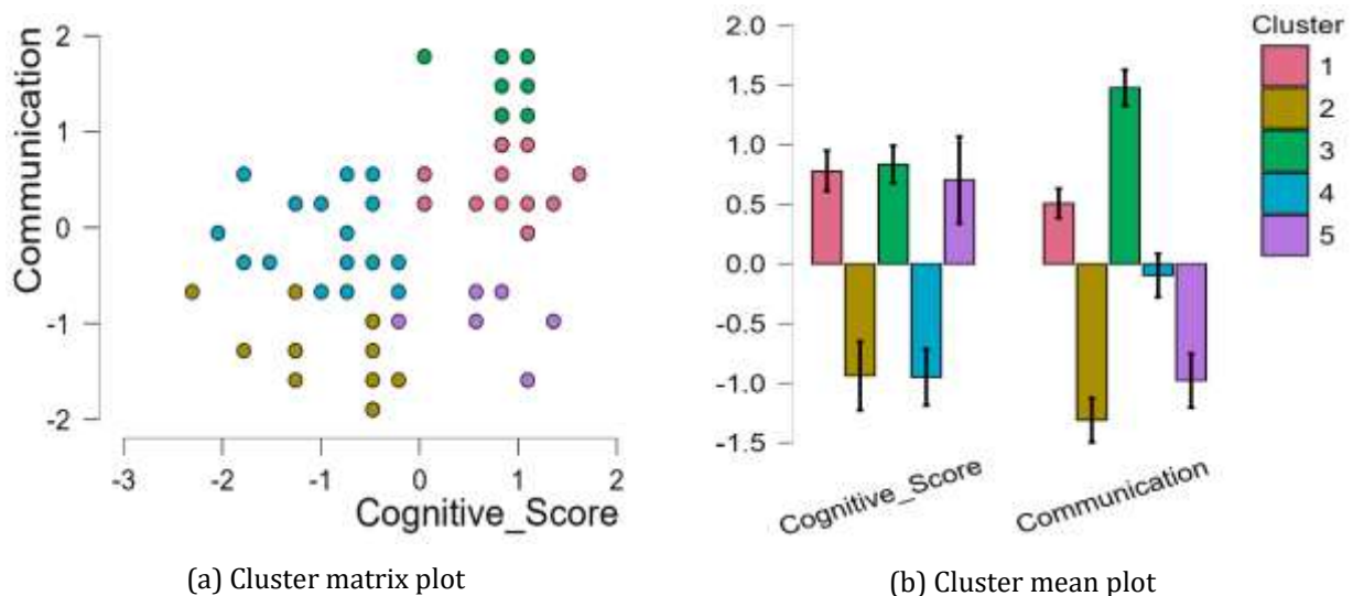
Figure 1. Cluster plots
