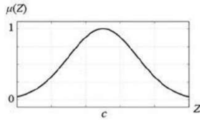
Figure 1. Gaussian Membership Function. (Gupta et al., 2023)
